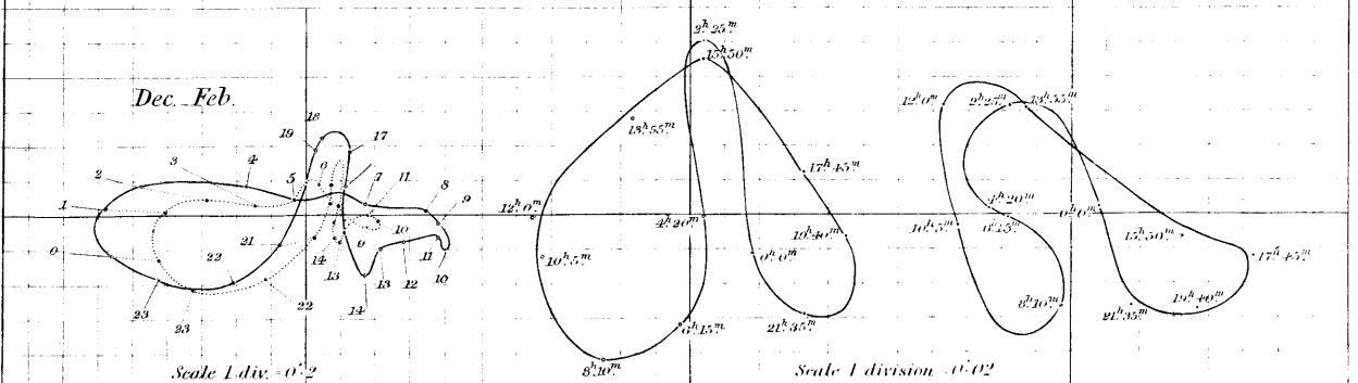
Motions with reference to the Moon's hour angles
