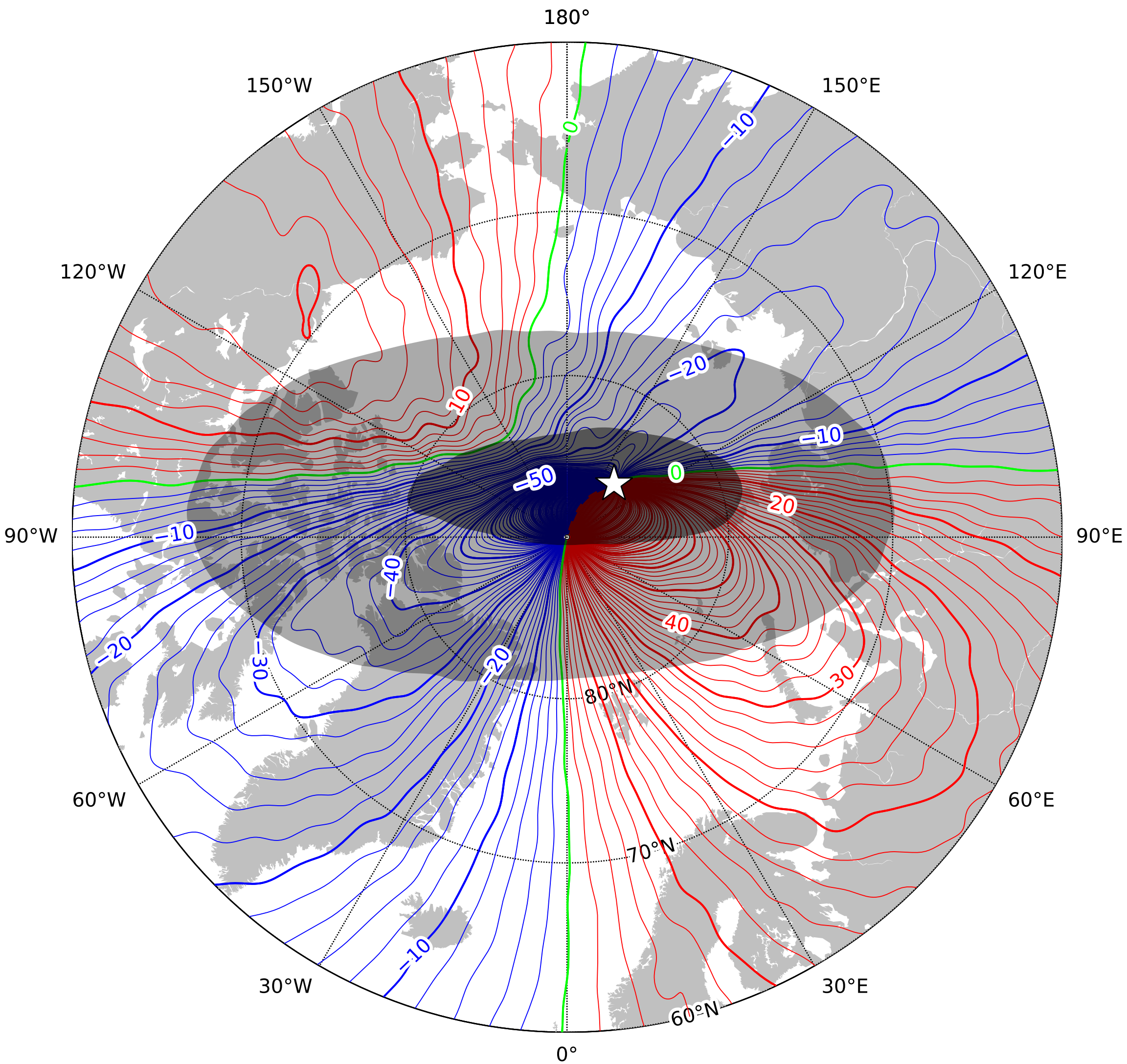
Declination (magnetic variation) in the region of the north pole at 2025.0 from the World Magnetic Model - High Resolution (WMMHR) 2025. Red - positive (east), blue - negative (west), green - zero (agonic line). Dashed red and blue line has 180^\circ declination. Contour interval is 2^\circ , white star is the location of a magnetic pole and the projection is Polar Stereographic. The black [grey] shaded regions around the poles correspond to the Blackout Zones [Caution Zones], i.e., regions where the horizontal component of the magnetic field H < 2000\text{nT} [ H < 6000\text{nT} ]. This is an example of an isogonic chart.
