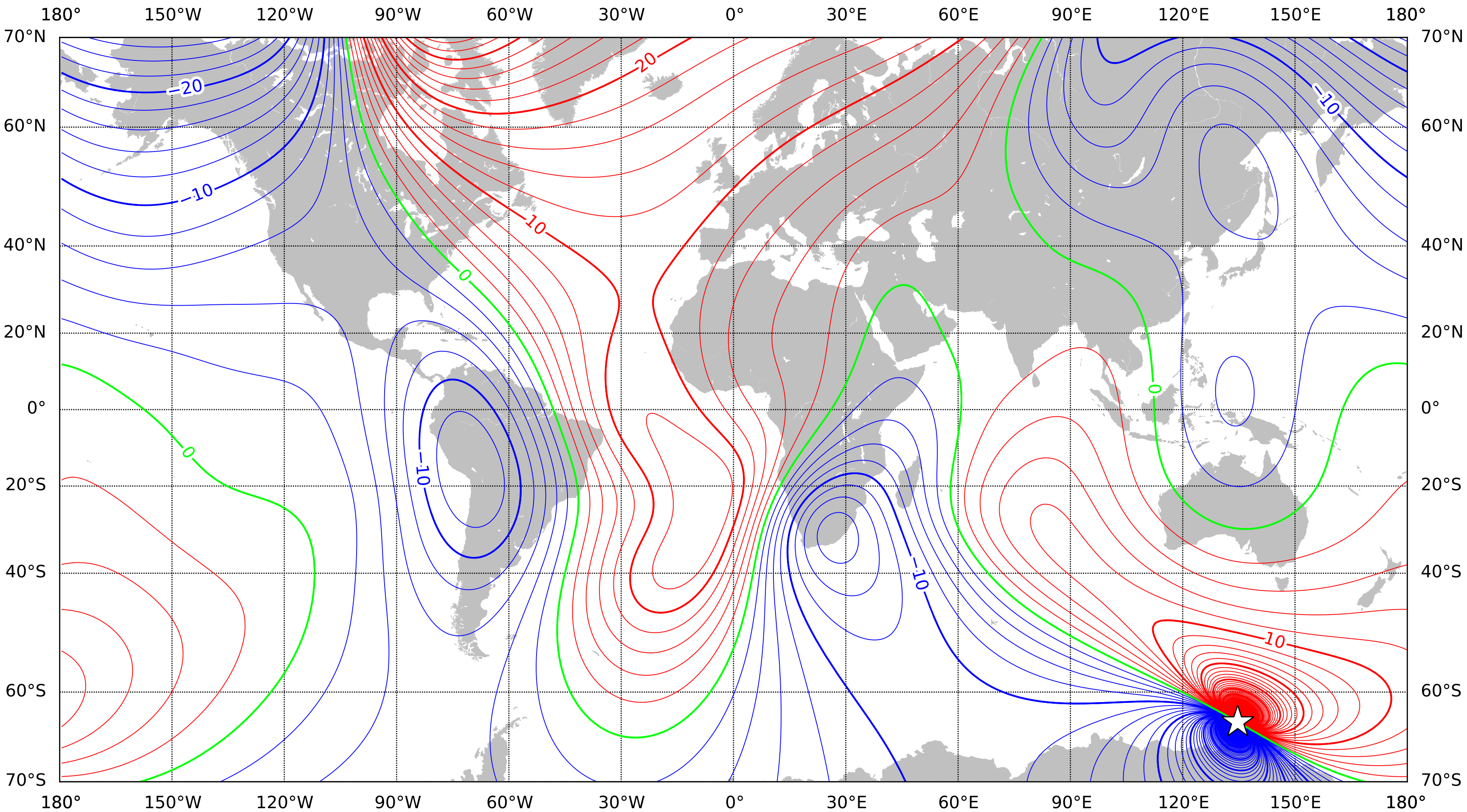
Annual rate of change of declination at 2027.5 from the World Magnetic Model - High Resolution (WMMHR) 2025 (core component only). Red - positive (easterly) change, blue - negative (westerly) change, green - zero change. Contour interval is 2°/year, white star is the location of a magnetic pole and the projection is Mercator. This is an example of an isoporic chart.
