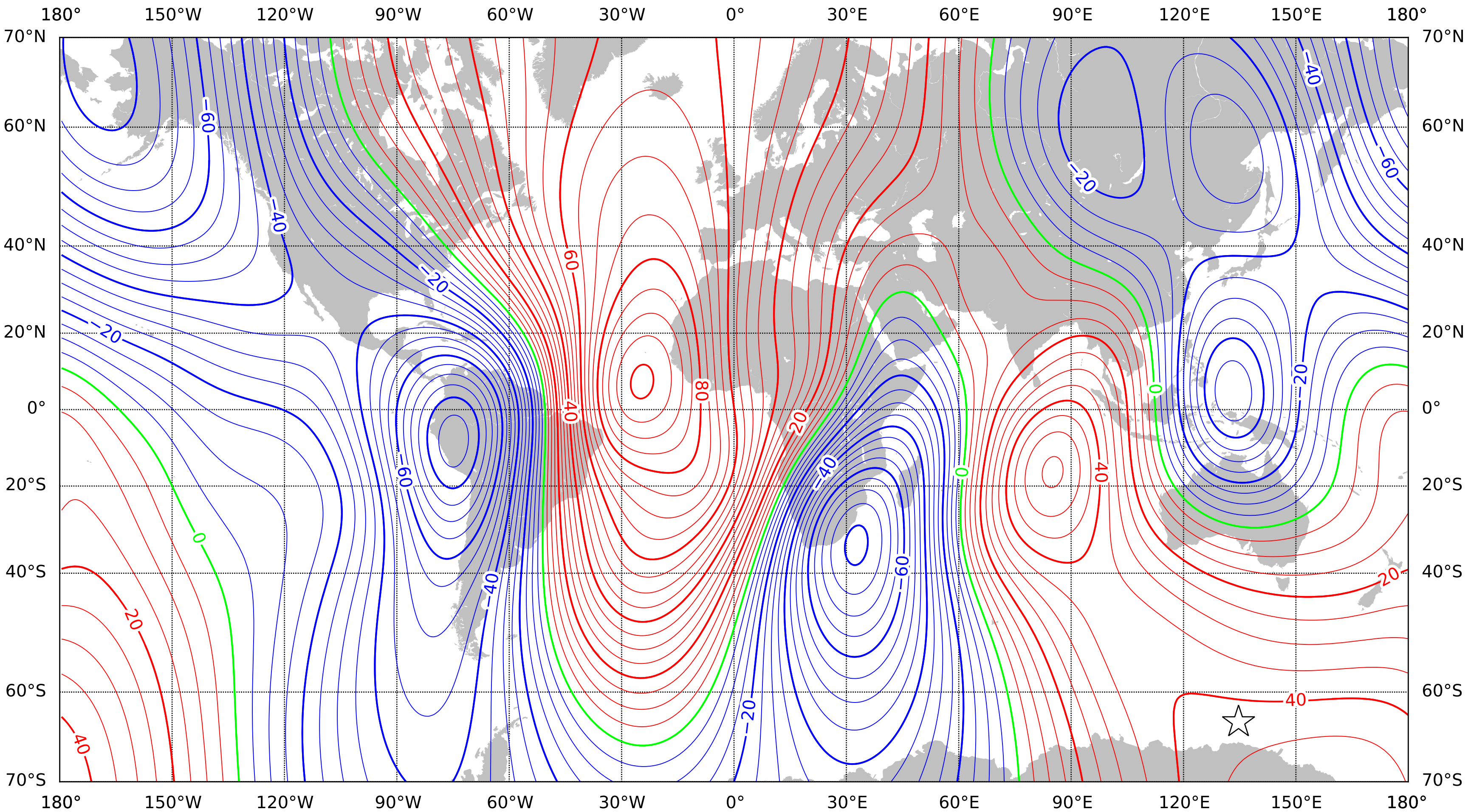
Annual rate of change of east component at 2027.5 from the World Magnetic Model - High Resolution (WMMHR) 2025 (core component only). Red - positive (easterly) change, blue - negative (westerly) change, green - zero change. Contour interval is 5nT/year, white star is the location of a magnetic pole and the projection is Mercator. This is an example of an isoporic chart. British Geological Survey © UKRI 2024
