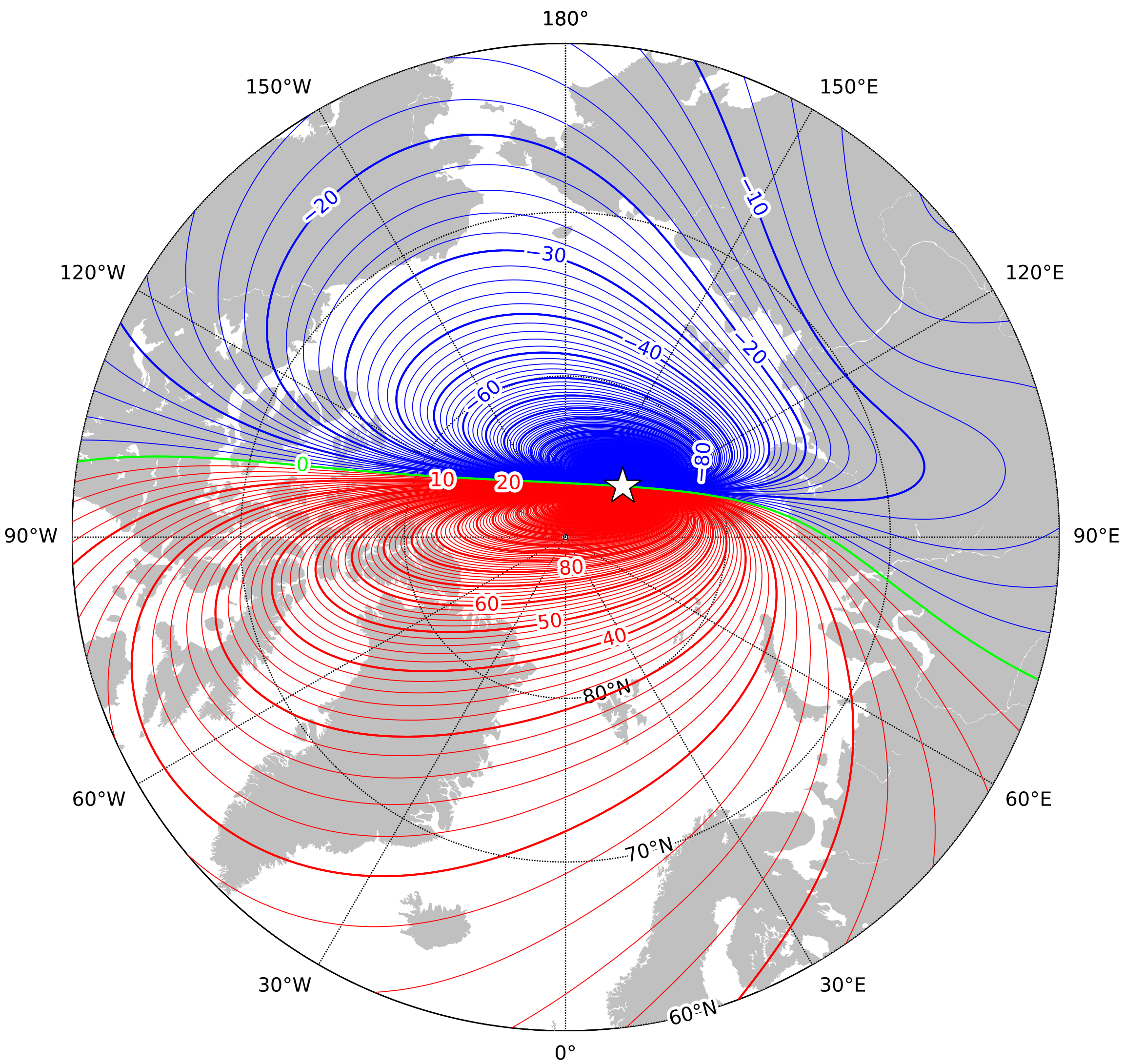
Annual rate of change of declination in the region of the north pole at 2027.5 from the World Magnetic Model - High Resolution (WMMHR) 2025 (core component only). Red - positive (easterly) change, blue - negative (westerly) change, green - zero change. Contour interval is 2'/year, white star is the location of a magnetic pole and the projection is Polar Stereographic. This is an example of an isoporic chart. British Geological Survey © UKRI 2024
