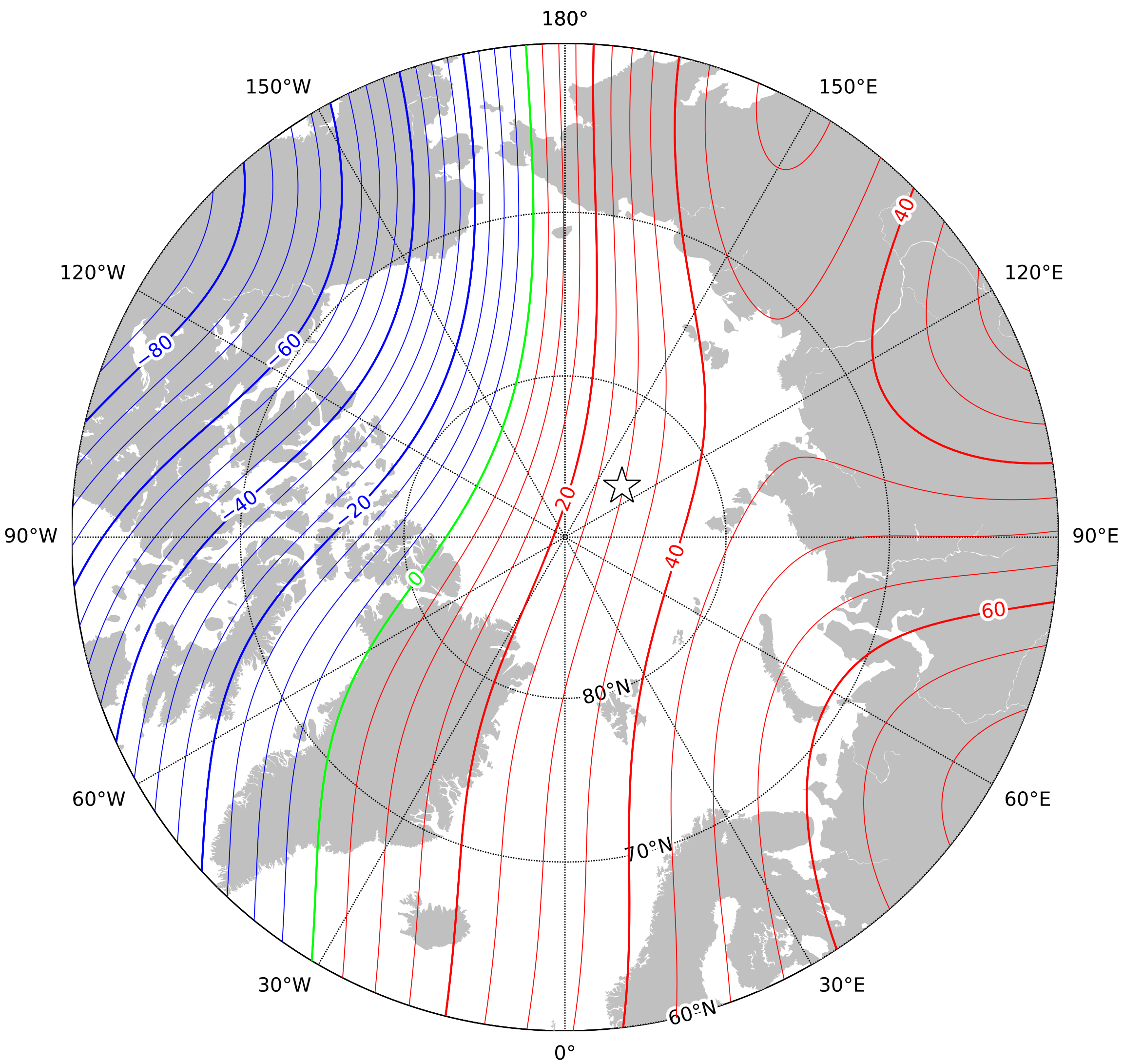
Annual rate of change of total intensity in the region of the north pole at 2027.5 from the World Magnetic Model (WMM) 2025. Red - positive change, blue - negative change, green - zero change. Contour interval is 5nT/year, white star is the location of a magnetic pole and the projection is Polar Stereographic. This is an example of an isoporic chart.
