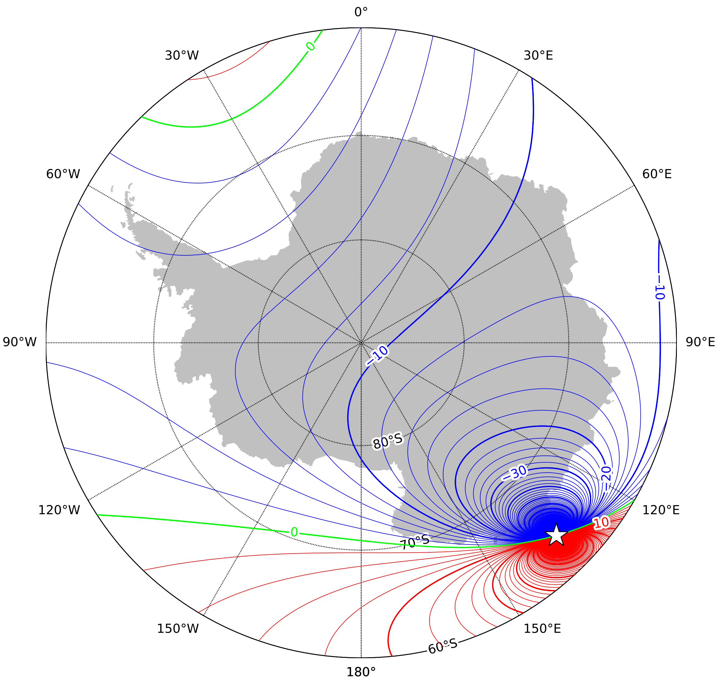
Annual rate of change of declination in the region of the south pole at 2027.5 from the World Magnetic Model (WMM) 2025. Red - positive (easterly) change, blue - negative (westerly) change, green - zero change. Contour interval is 2'/year, white star is the location of a magnetic pole and the projection is Polar Stereographic. This is an example of an isoporic chart. British Geological Survey © UKRI 2024
