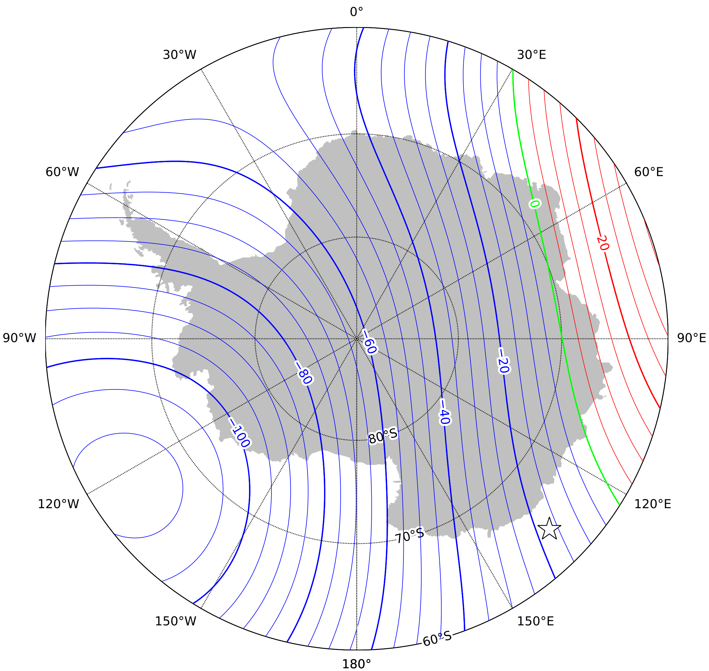
Annual rate of change of total intensity in the region of the south pole at 2027.5 from the World Magnetic Model (WMM) 2025. Red - positive change, blue - negative change, green - zero change. Contour interval is 5nT/year, white star is the location of a magnetic pole and the projection is Polar Stereographic. This is an example of an isoporic chart. British Geological Survey © UKRI 2024
